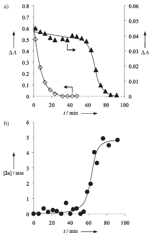
Figure 2. Time profiles of a) the absorbance at 360 ( \diamond ) and 700 nm ( \blacktriangle ) and b) formation of 2a from the reaction of I with 1a under argon (1 atm). Reaction conditions: I (4 mM), 1a (200 mM), benzonitrile (1 mL), 373 K. Changes in the UV/Vis spectra are shown in the Supporting Information. The concentration of 2a was determined by GC analysis.
